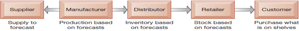
Push-Based Model
