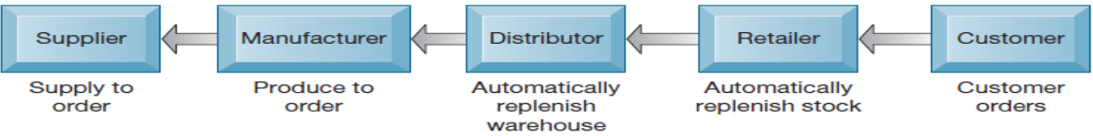
Pull-Based Model
